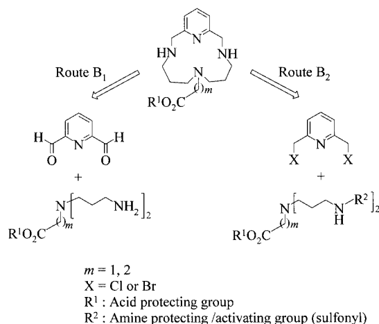
Scheme 3. Macrocyclisation processes envisaged for the preparation of regioselectively N -functionalised azapyridinomacrocycles 2c and 2d
