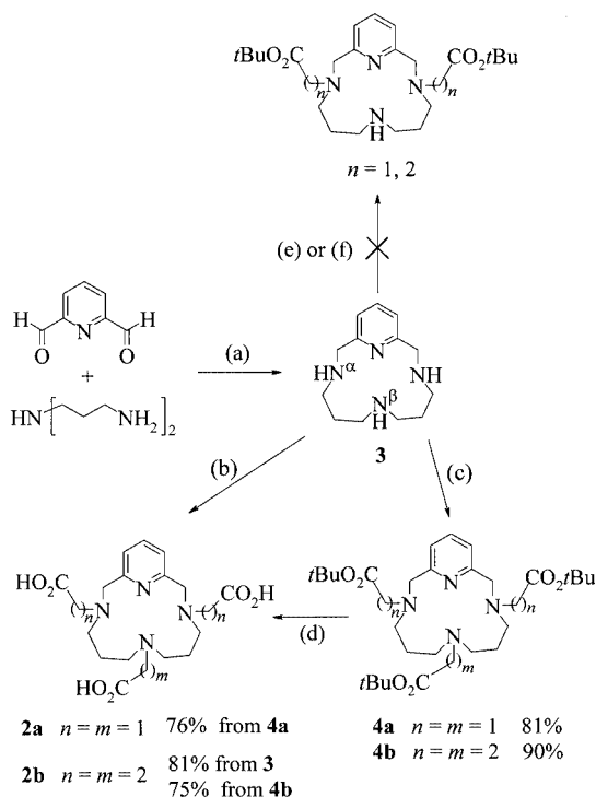
Scheme 2. Synthesis of macrocycles 2a and 2b by Route A; reagents and conditions: (a) see ref. [8] ; (b) acrylic acid, H 2 O, 70 °C, overnight; (c) for 4a : tert -butyl bromoacetate (12 equiv.), Ag 2 CO 3 (2.5 equiv.), THF, room temp., 1 h; for 4b : tert -butyl acrylate (13 equiv.), MeOH, 70 °C, 40 h; (d) HCl, Et 2 O; (e) tert -butyl bromoacetate (2 equiv.), Ag 2 CO 3 (2 equiv.), THF, room temp., 7 d or tert -butyl bromoacetate (2.5 equiv.), NaOH (2.5 equiv.), CH 2 Cl 2 /H 2 O, room temp., 16 h; (f) tert -butyl acrylate (2 equiv.), MeOH, 70 °C, 20 h
