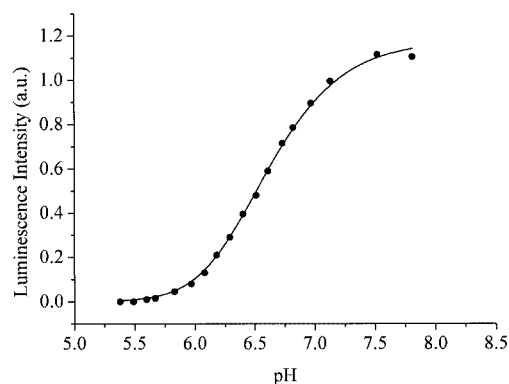
Figure 6. Binding curve resulting from monitoring of the luminescence intensity (615 nm) of samples containing 50.00 \mu\text{M} of ligand 2a and \text{EuCl}_3 (56.25 \mu\text{M} ) as a function of the pH (0.015 M MES-buffered solutions with 0.085 M of KCl); the luminescence results from UV light excitation at 262 nm; the full circles represent actual data points and the solid line represents the theoretical fit of data with \log K^{\text{Eu}} = 9.54
