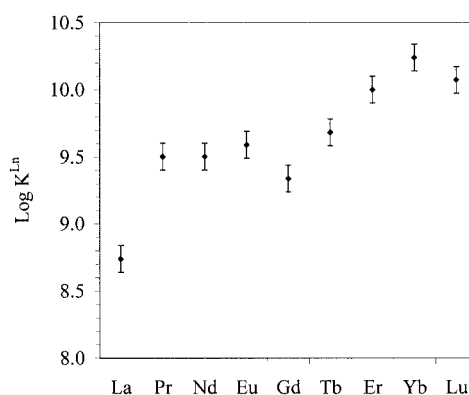
Figure 8. Stability constants of lanthanide complexes formed with ligand 2a
