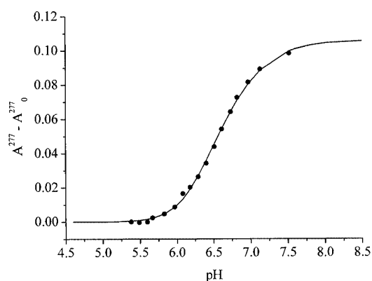
Figure 7. Binding curve resulting from monitoring of the relative absorbance at 277 nm ( A^{277} - A_0^{277} ) of samples containing 50.00 \mu\text{M} of ligand 2a and \text{EuCl}_3 (56.25 \mu\text{M} ) as a function of the pH (0.015 M MES-buffered solutions with 0.085 M of KCl); the full circles represent actual data points and the solid line represents the theoretical fit of data with \log K^{\text{Eu}} = 9.59
