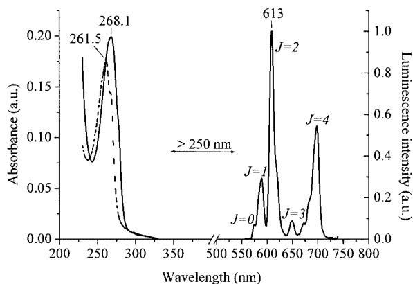
Figure 3. Absorption spectra of free ligand 2a (dotted line) and of ligand 2a in the presence of \text{EuCl}_3 (solid line, 200–320 nm) in HEPES-buffered aqueous medium (pH = 8.0); sensitised emission spectrum (solid line, 550–750 nm) obtained by irradiation at 262 nm of the previous buffered aqueous solution of ligand 2a and \text{EuCl}_3
