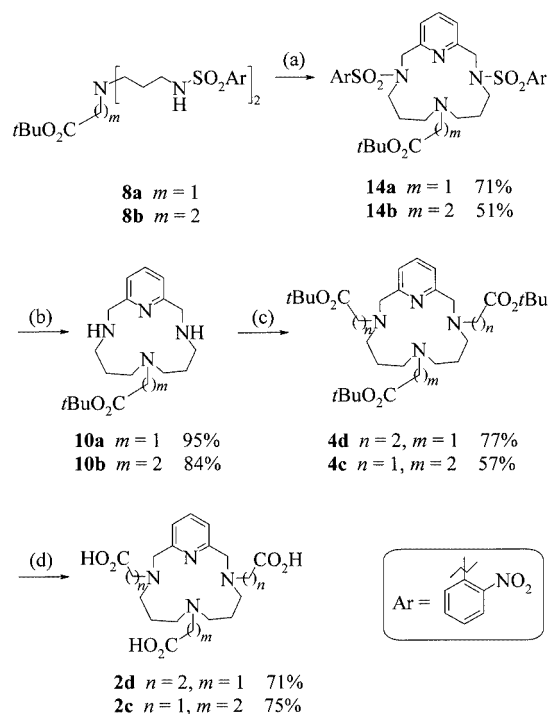
Scheme 5. Synthesis of azapyridinomacrocycles 2c and 2d by route B2 ; reagents and conditions: (a) 2,6-bis(bromomethyl)pyridine (1.2 equiv.), \text{Na}_2\text{CO}_3 (5 equiv.), DMF, 100 °C, 1 d; (b) PhSH (3.3 equiv.), \text{Na}_2\text{CO}_3 (10 equiv.), DMF, room temp., 5–15 h; (c) for 4d : tert -butyl acrylate/MeOH (6:1), 70 °C, overnight; for 4c : (i) tert -butyl bromoacetate (5.5 equiv.), \text{Ag}_2\text{CO}_3 (0.3 equiv.), THF, room temp., 1 h; (ii) HCl; (iii) \text{Na}_2\text{S} ; (d) HCl, \text{Et}_2\text{O} , room temp., overnight
