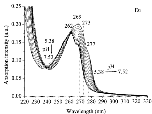
Figure 5. UV absorbance spectra of ligand 2a (50.00 \mu\text{M} ) in the presence of \text{EuCl}_3 (56.25 \mu\text{M} ) in MES-buffered aqueous medium (0.015 M) and KCl (0.085 M); the pH varies from 5.38 to 7.52
