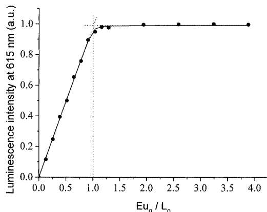
Figure 4. Binding curve resulting from monitoring of the luminescence intensity (615 nm) of samples containing 37.4 \mu\text{M} of ligand 2a ( L_0 ) and varying amounts of \text{EuCl}_3 ( \text{Eu}_0 : 0–150 \mu\text{M} ) in 0.085 M of KCl and 0.015 M HEPES-buffered medium (pH = 8.0); the luminescence results from a UV light excitation at 262 nm; the full circles represent actual data points and the solid line represents the theoretical fit of data with \log K^{\text{Eu}} = 9.54 and I_{\text{max.}} = 0.997
