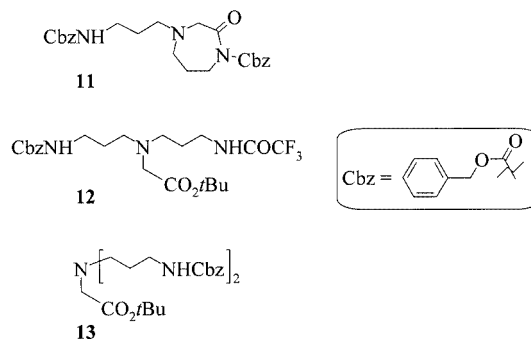
Figure 2. Derivatised side products recovered from the trifluoroacetamides 7a and 7b cleavage step
