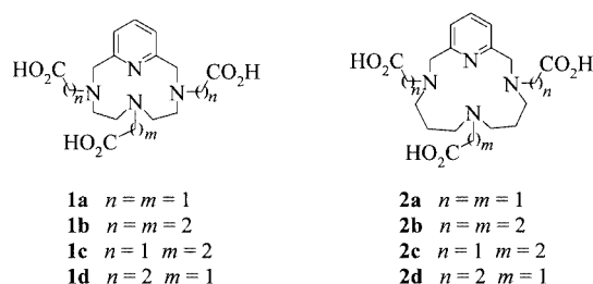
Figure 1. Azapyridinomacrocycles as ligand for lanthanide cations
